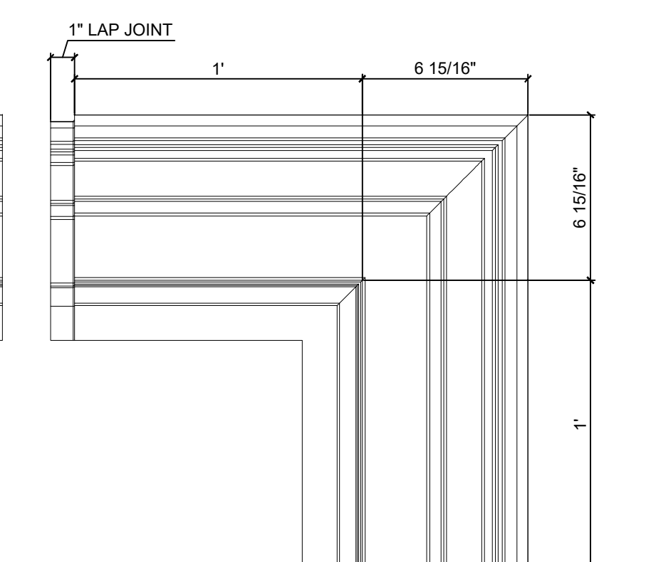
10 CR109x8 Outside Corner Under Side SCALE 1:1
