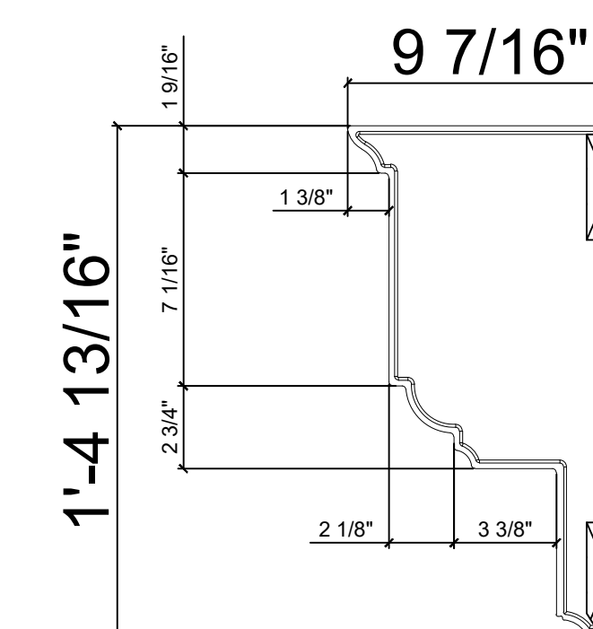
7 CR109x8 Cross Section SCALE 1:1
