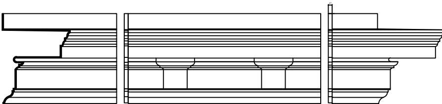
CR130x4 Elevation of Inside Corner SCALE 1:1
