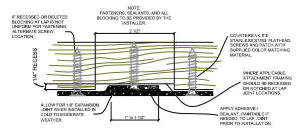
Typical Lap Joint Detail Not to Scale
