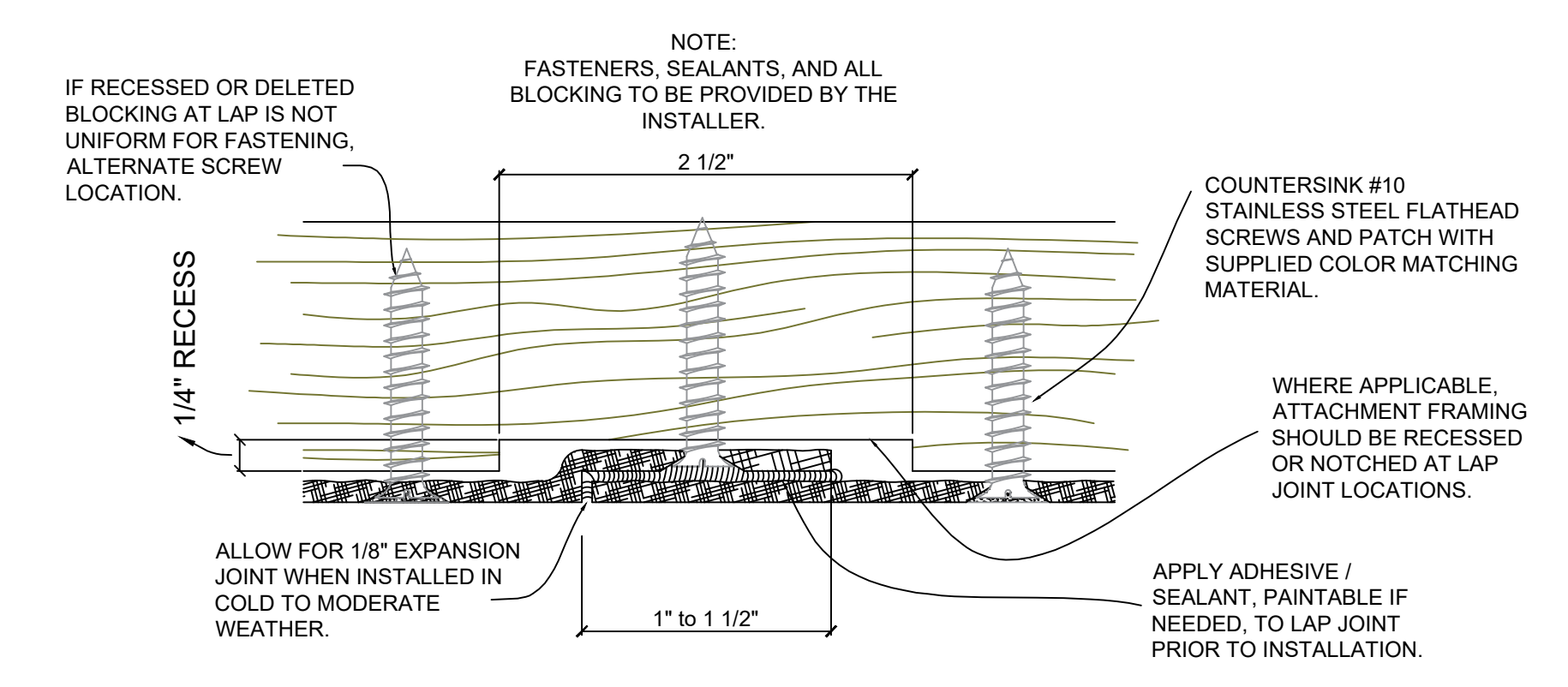
11 Typical Lap Joint Detail Not to Scale
