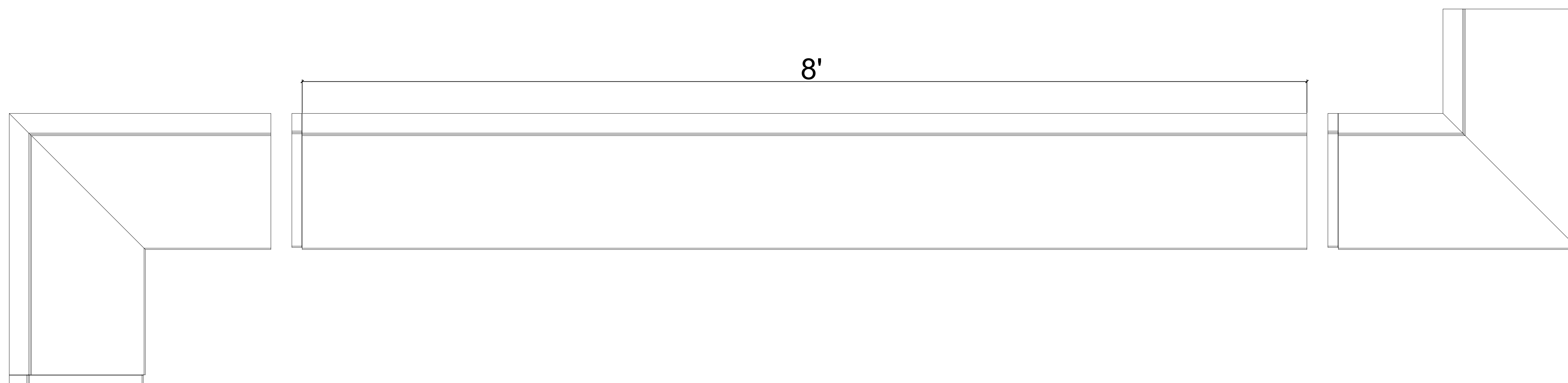
1 CR113x8 Inside Corner Top View SCALE 1:1
