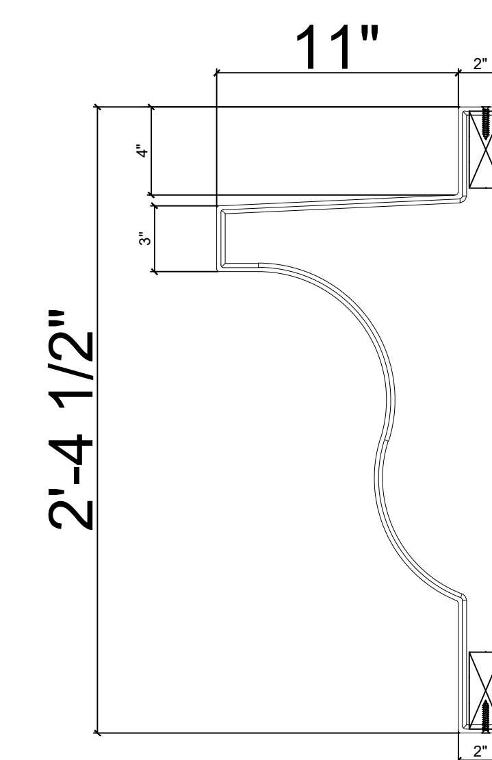
7 CR113x8 Cross Section SCALE 1:1
