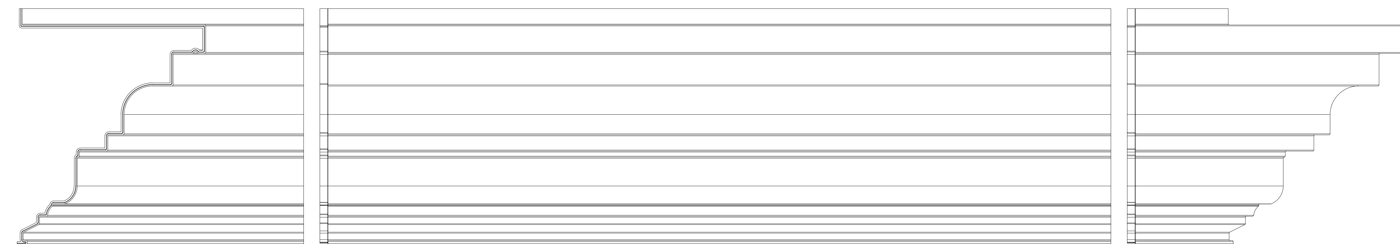
4 CR114x8 Elevation of Outside Corner SCALE 1:1
