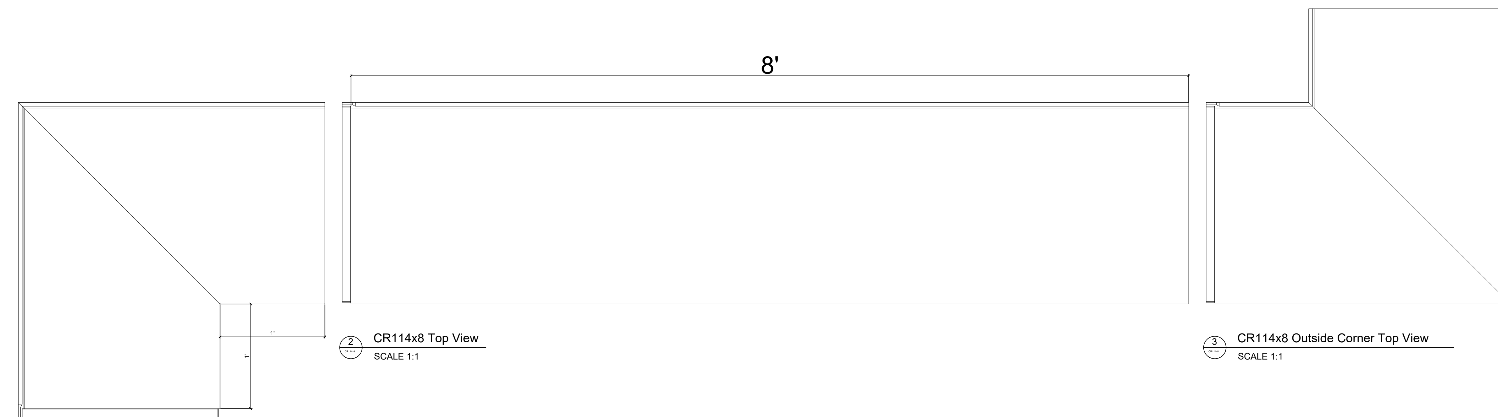
1 CR114x8 Inside Corner Top View SCALE 1:1
