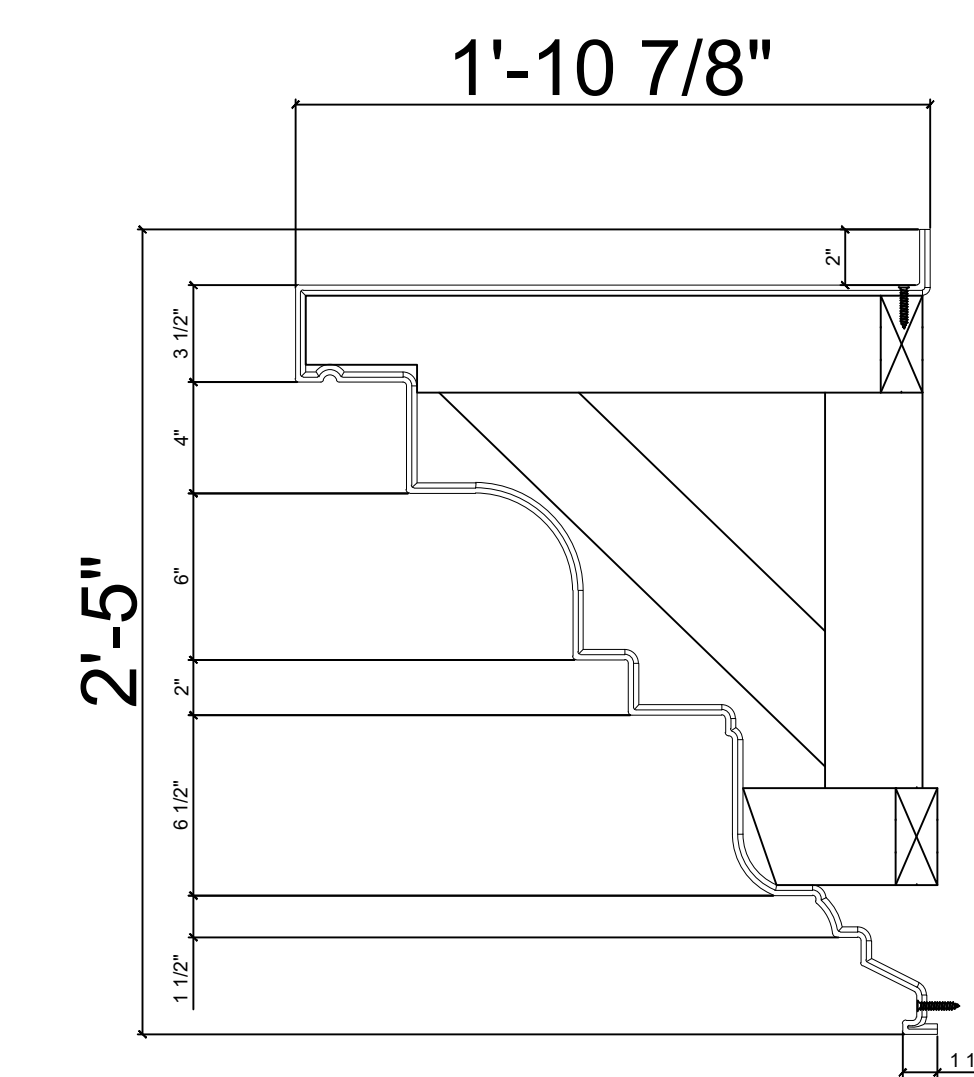
7 CR114x8 Cross Section SCALE 1:1
